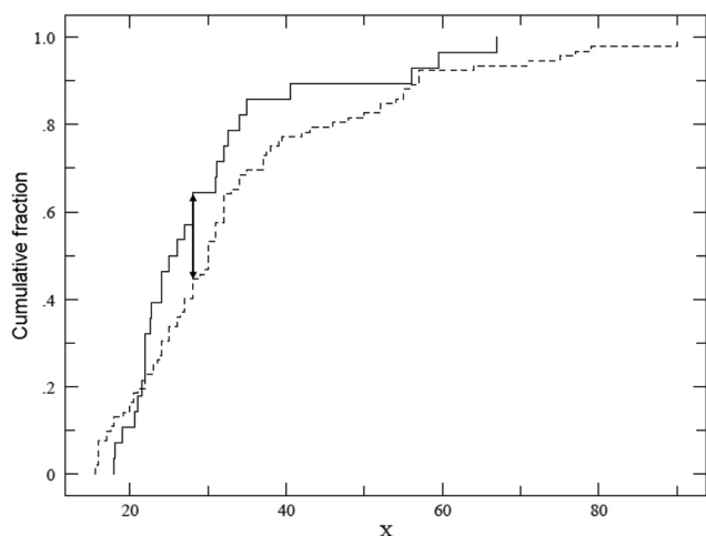
Figure 5. KS test comparison cumulative fraction plot for adult individuals of S. asoca from private forest versus protected area.
